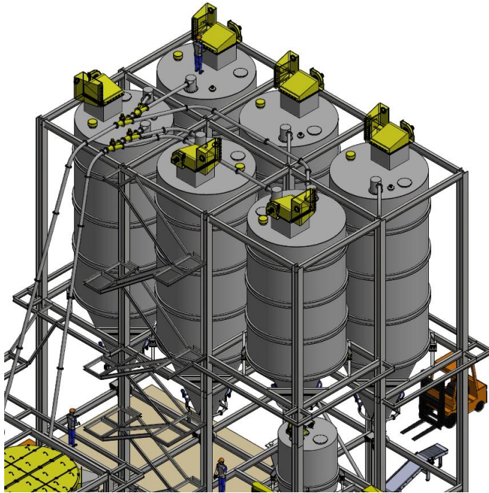
Customized Mortar Storage Silo
